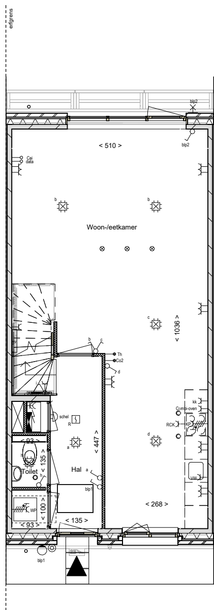
00 begane grond
